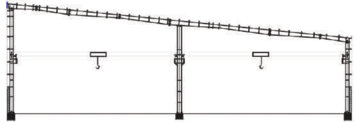
MULTI SPAN MONOSLOPE FRAME
