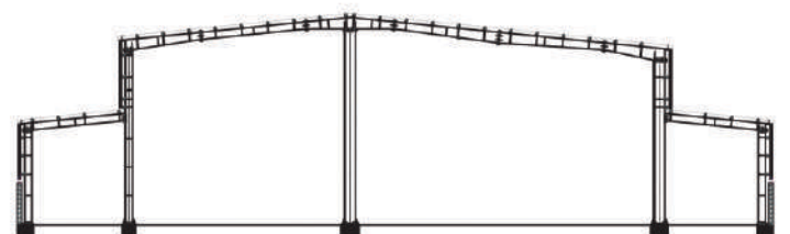
MULTI SPAN FRAME WITH LEAN TO STRUCTURE
