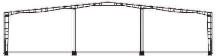
MULTI SPAN FRAME WITHOUT CRANE
