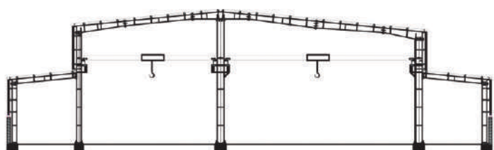
MULTI SPAN FRAME WITH LEAN TO STRUCTURE MULTI SPAN FRAME WITH CRANE
